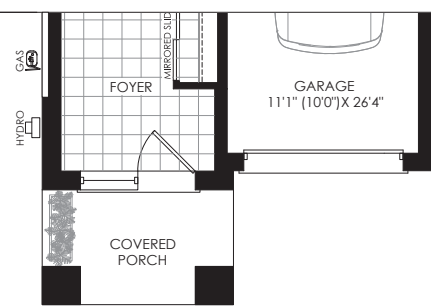
PARTIAL GROUND FLOOR PLAN ELEV. 'H'
