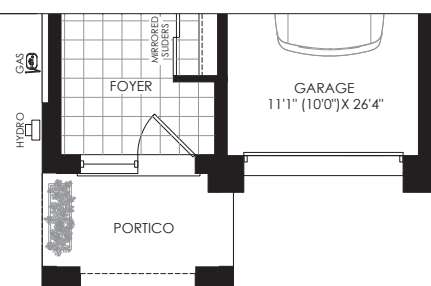
PARTIAL GROUND FLOOR PLAN ELEV. 'E'
