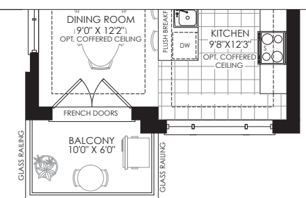
PARTIAL SECOND FLOOR PLAN ELEV. 'E'
