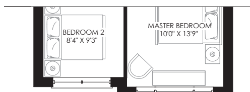
PARTIAL THIRD FLOOR PLAN ELEV. 'E' WITH ROOF TOP TERRACE STD. & FLEX PLAN
