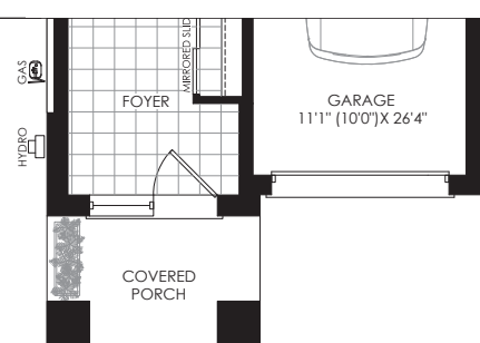
PARTIAL GROUND FLOOR PLAN ELEV. 'I'
