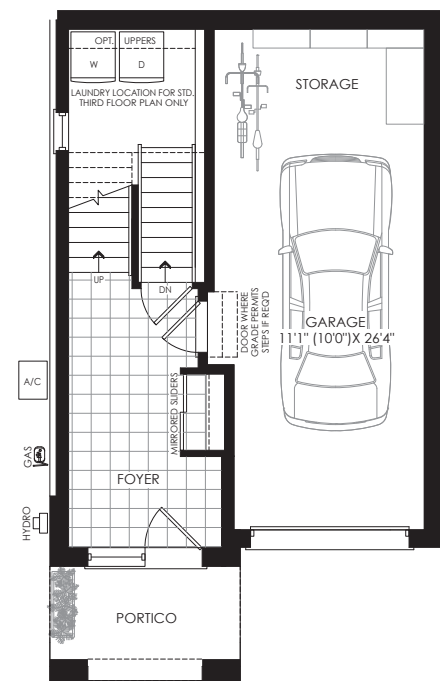
GROUND FLOOR PLAN ELEV. 'D'
