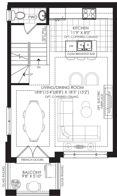
FLEX SECOND FLOOR PLAN ELEV. 'D'
