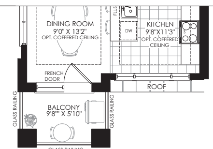
PARTIAL SECOND FLOOR PLAN ELEV. 'H'
