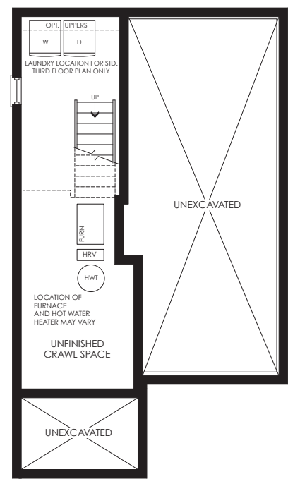
CRAWL SPACE PLAN ELEV. 'D'
